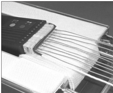
Data logger with TX2040A antenna correctly routed across thermocouple plugs.
